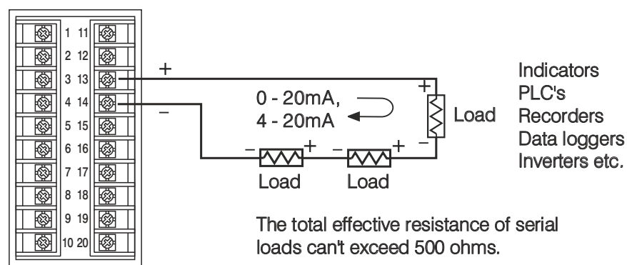
Retransmit Current
