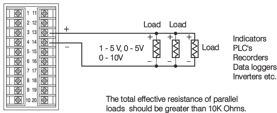
Retransmit Voltage
