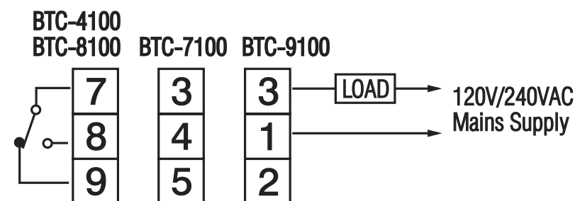
Figure 2.19 Alarm Output to Drive Load
