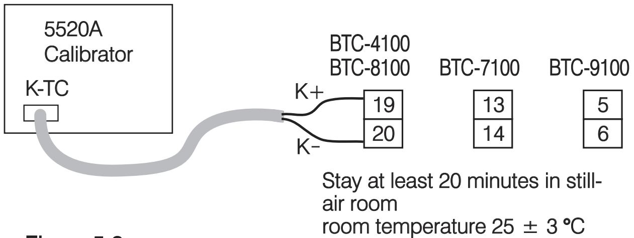
Figure 5.2 Cold Junction Calibration Setup
