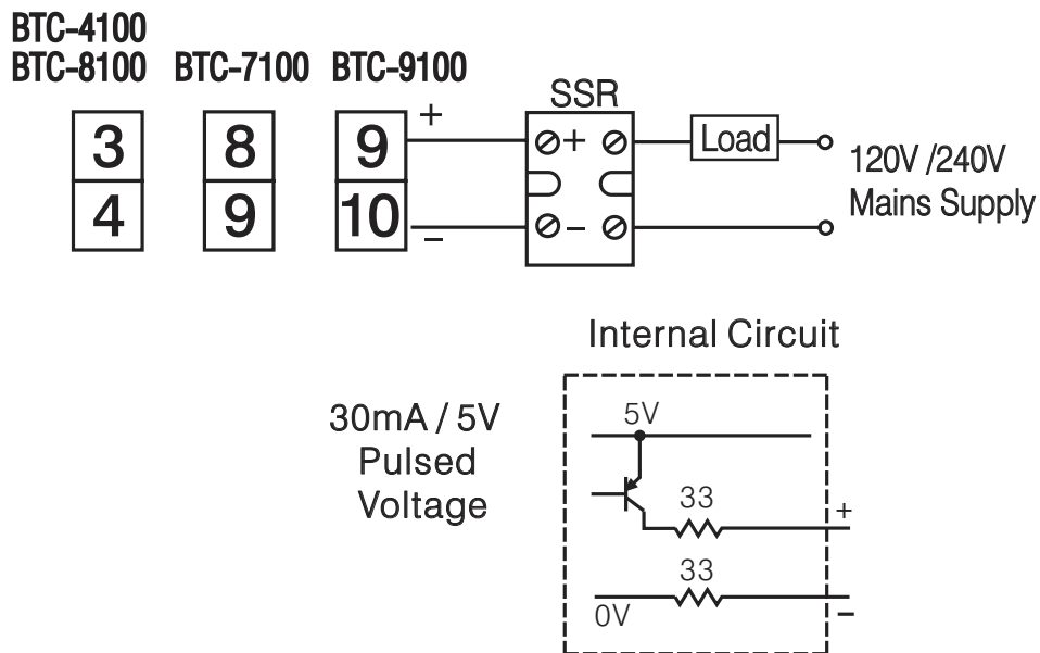
Figure 2.11 Output 1 Pulsed Voltage to Drive SSR
