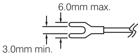
Figure 2.3 Lead Termination for BTC-9100
