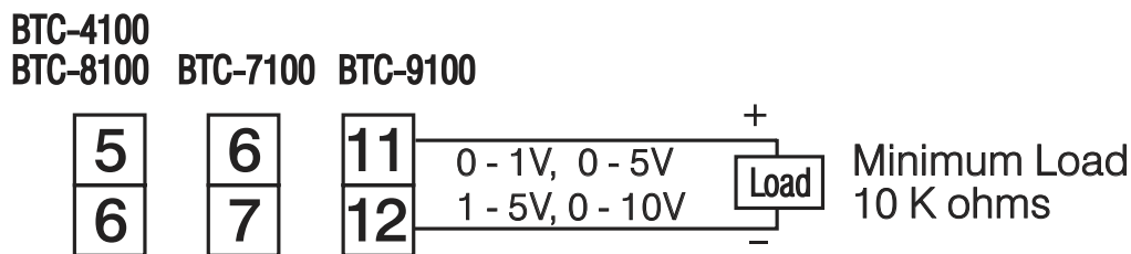
Figure 2.18 Output 2 Linear Voltage
