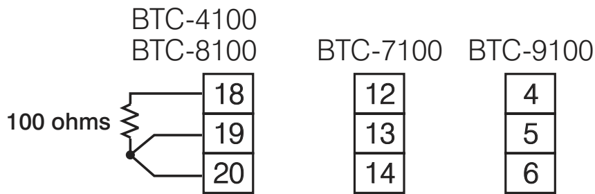
Figure 5.1 RTD Calibration
