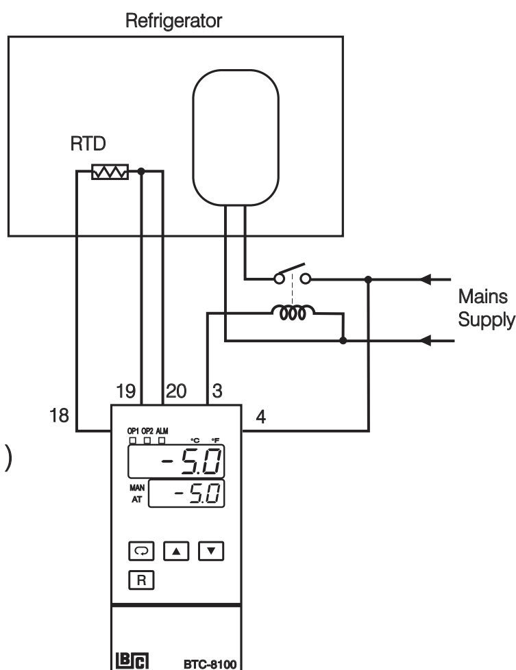
Figure 4.2 Cooling Control Example
