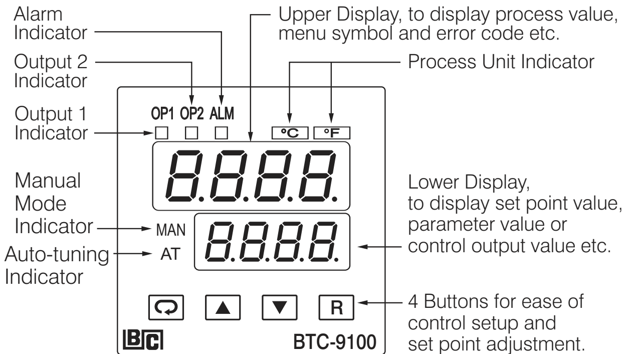
Figure 1.3 Front Panel Description
