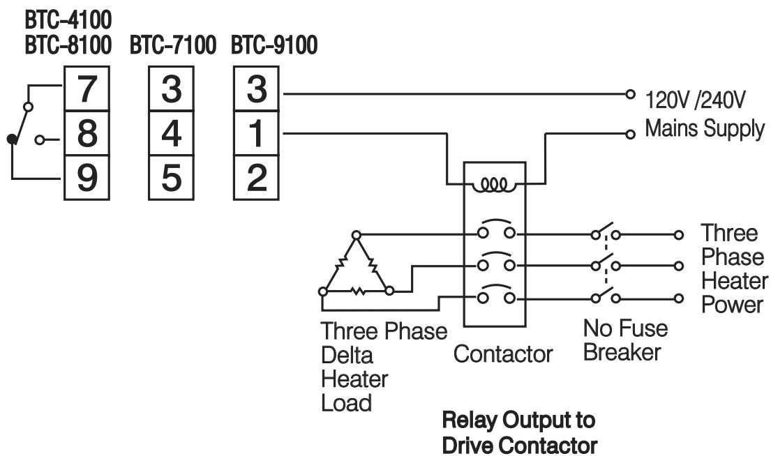
Figure 2.20 Alarm Output to Drive Contactor
