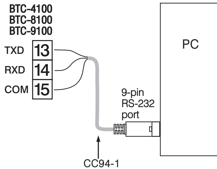
Figure 2.22 RS-232 Wiring
