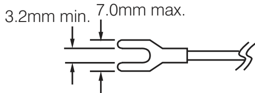
Figure 2.2 Lead Termination for BTC-4100, BTC-8100 and BTC-7100
