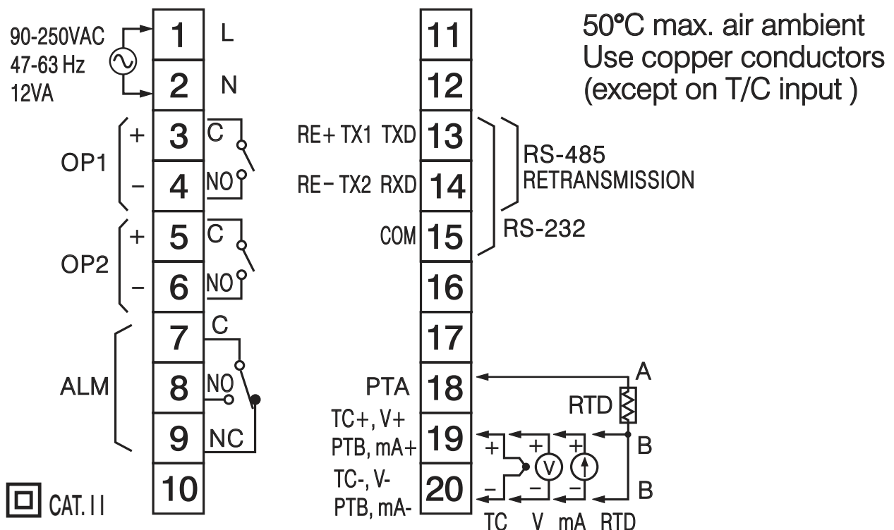
Figure 2.4 Rear Terminal Connection for BTC-4100 and BTC-8100
