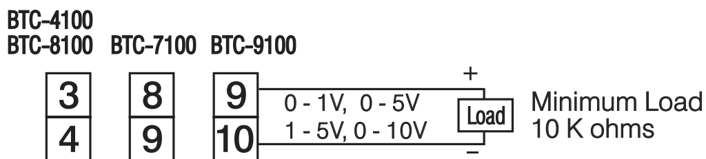
Figure 2.13 Output 1 Linear Voltage
