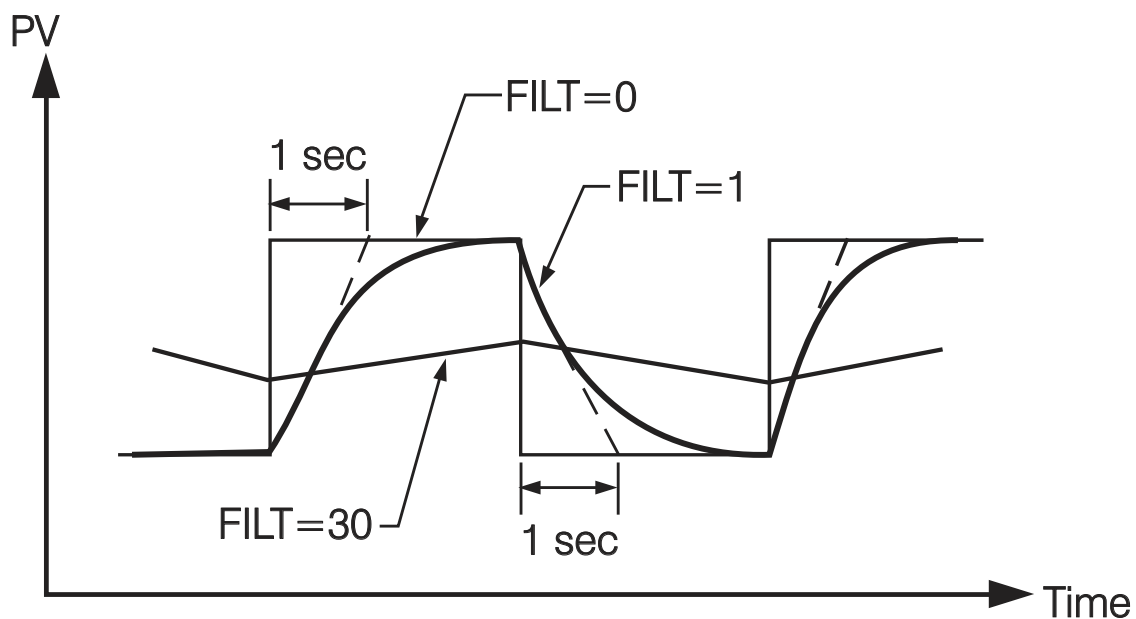
Figure 3.8 Filter Characteristics
