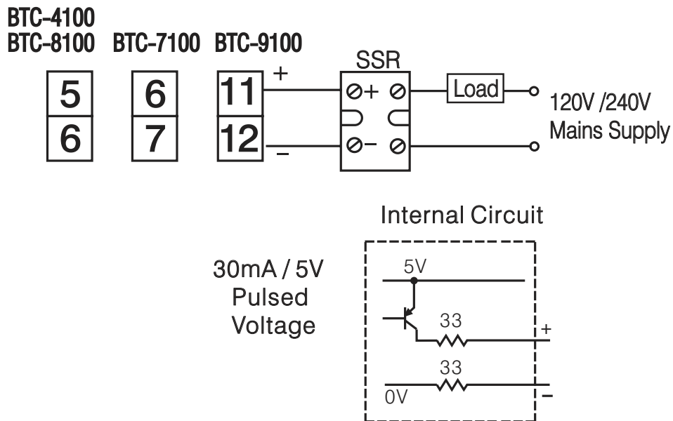
Figure 2.16 Output 2 Pulsed Voltage to Drive SSR
