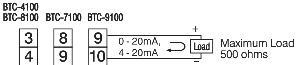
Figure 2.12 Output 1 Linear Current
