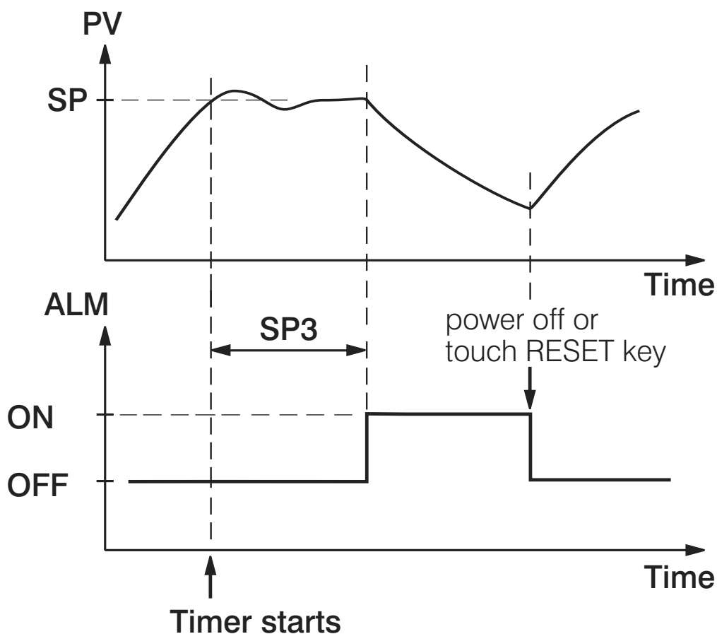
Figure 3.6 Dwell Timer Function
