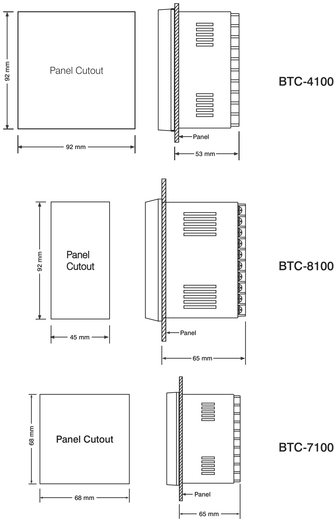
Figure 2.1 Mounting Dimensions
