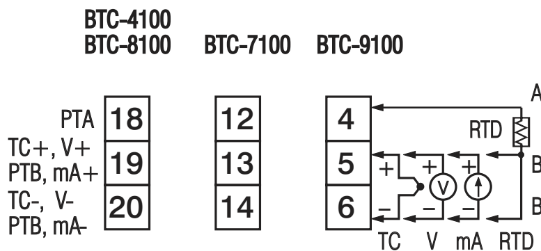
Figure 2.8 Sensor Input Wiring
