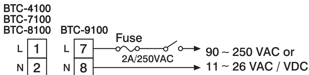
Figure 2.7 Power Supply Connections
