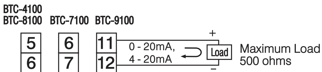
Figure 2.17 Output 2 Linear Current
