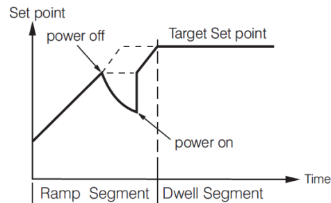
Power failure recovery from profile at Ramp segment
