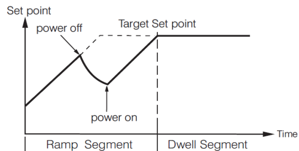
Power failure recovery from PV at Ramp Segment
