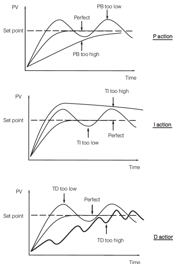
Effects of PID Adjustment
