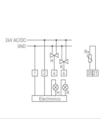
Connecting diagram RTR-S013
