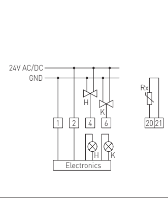
Connecting diagram RTR-S012
